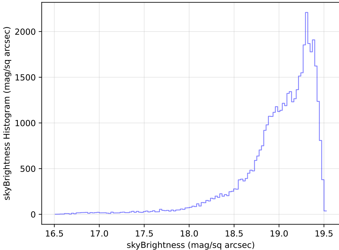
too_elab_r8_d3_ugrizy_v3.4_10yrs Yr 1 z band: skyBrightness Histogram
