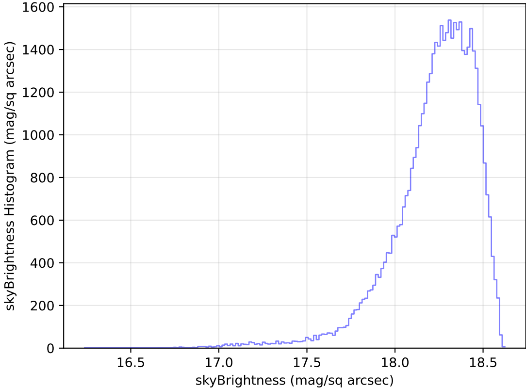
too_elab_r8_d3_ugrizy_v3.4_10yrs Yr 1 y band: skyBrightness Histogram
