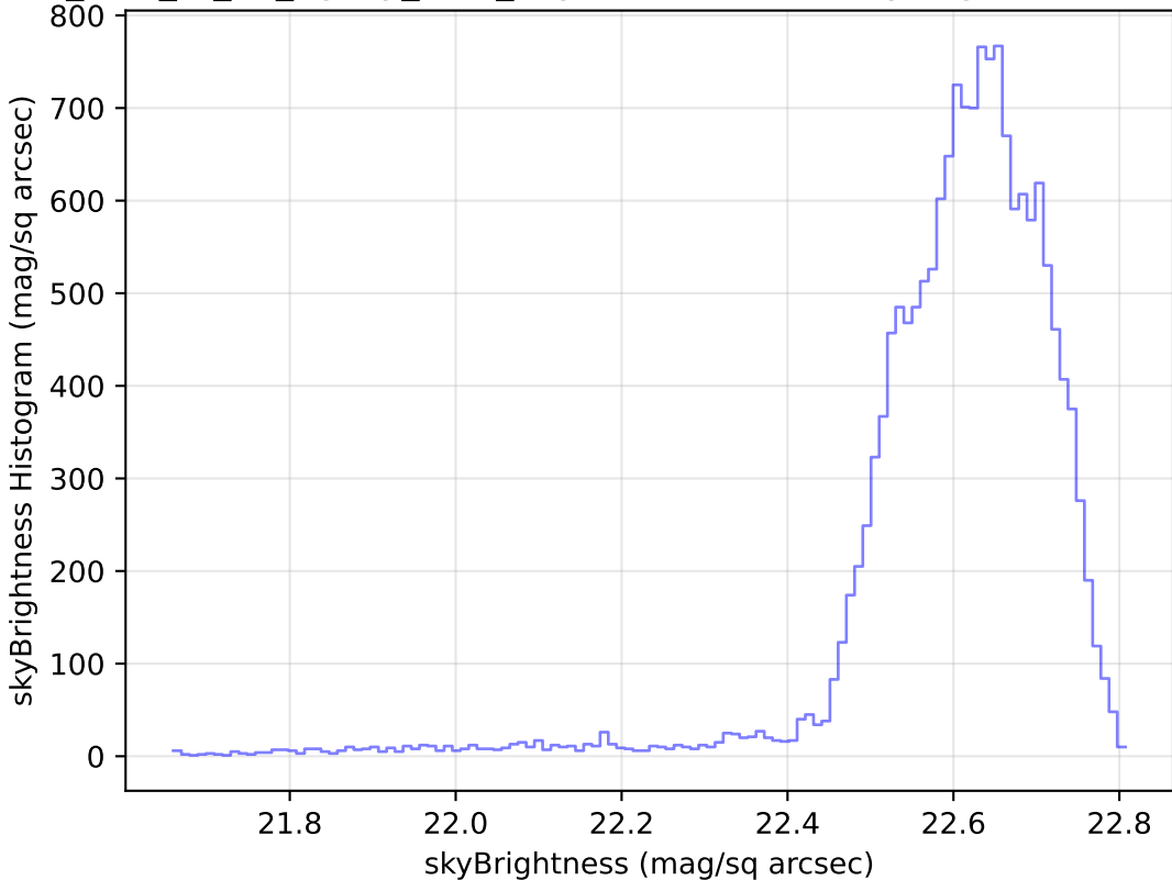
too_elab_r8_d3_ugrizy_v3.4_10yrs Yr 1 u band: skyBrightness Histogram
