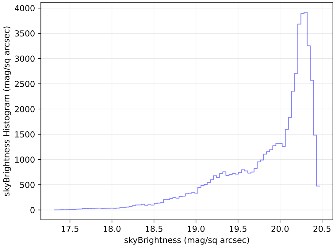
too_elab_r8_d3_ugrizy_v3.4_10yrs Yr 1 i band: skyBrightness Histogram
