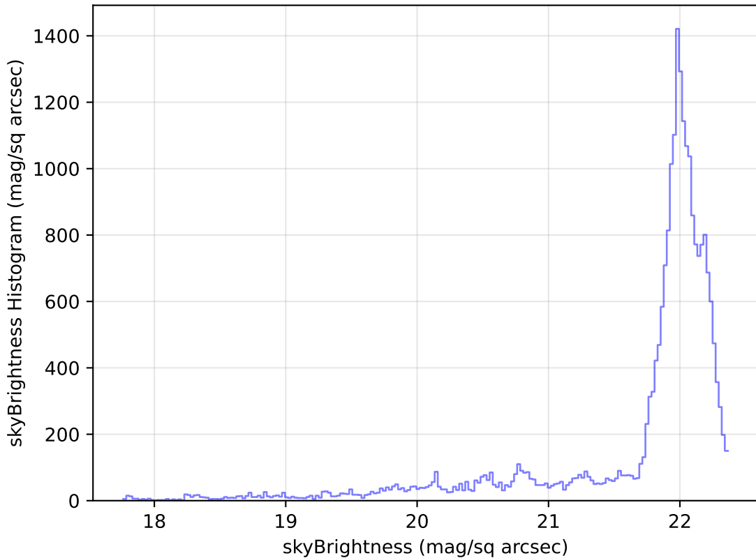
too_elab_r8_d3_ugrizy_v3.4_10yrs Yr 1 g band: skyBrightness Histogram
