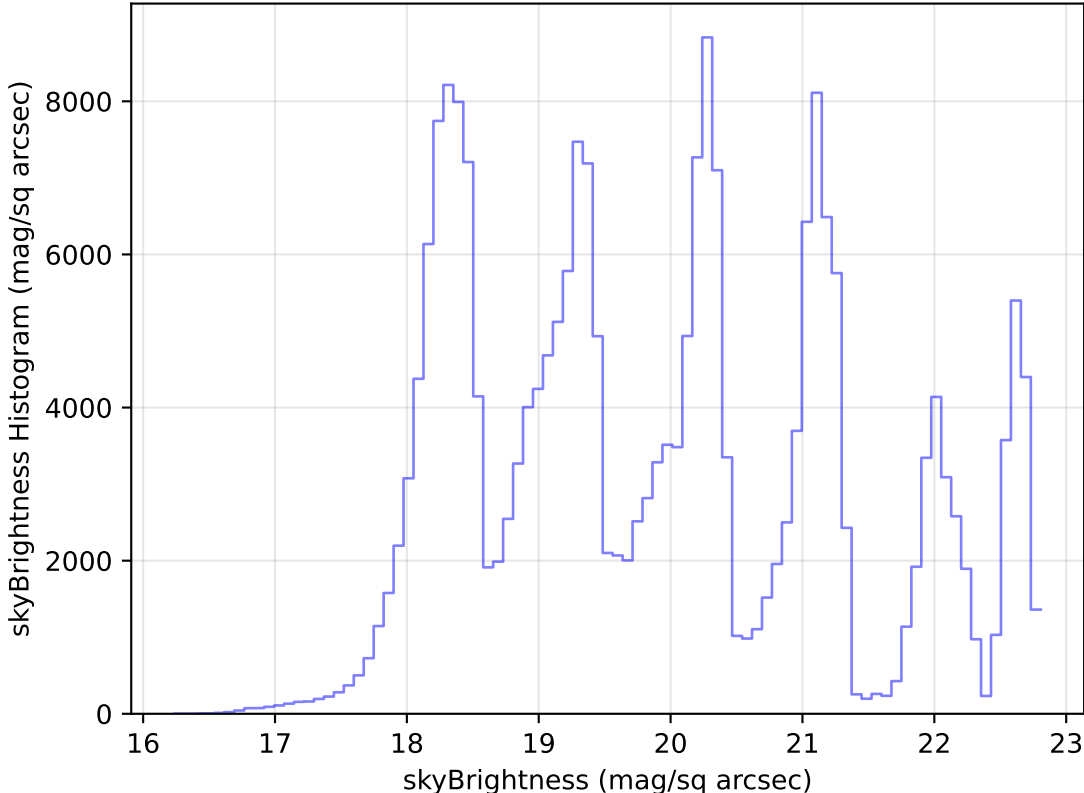
too_elab_r8_d3_ugrizy_v3.4_10yrs Yr 1 all bands: skyBrightness Histogram
