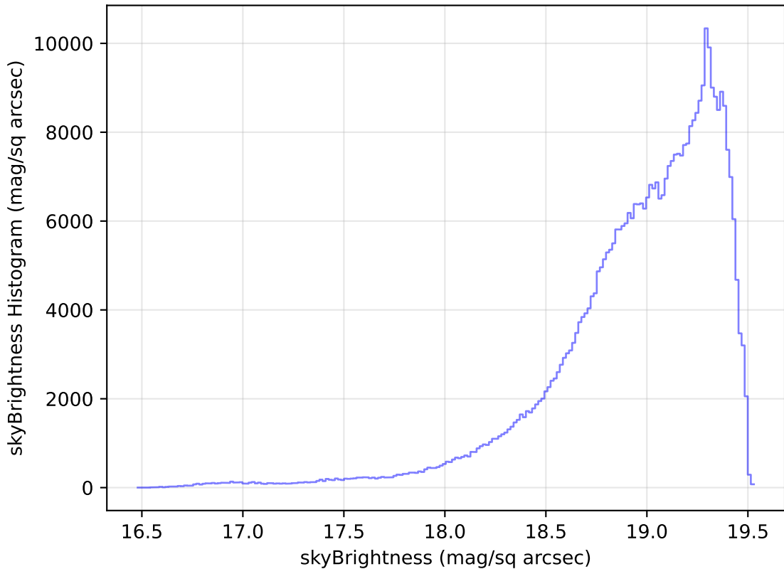
too_elab_r8_d3_ugrizy_v3.4_10yrs WFD z band: skyBrightness Histogram
