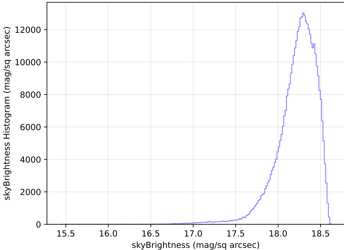
too_elab_r8_d3_ugrizy_v3.4_10yrs WFD y band: skyBrightness Histogram
