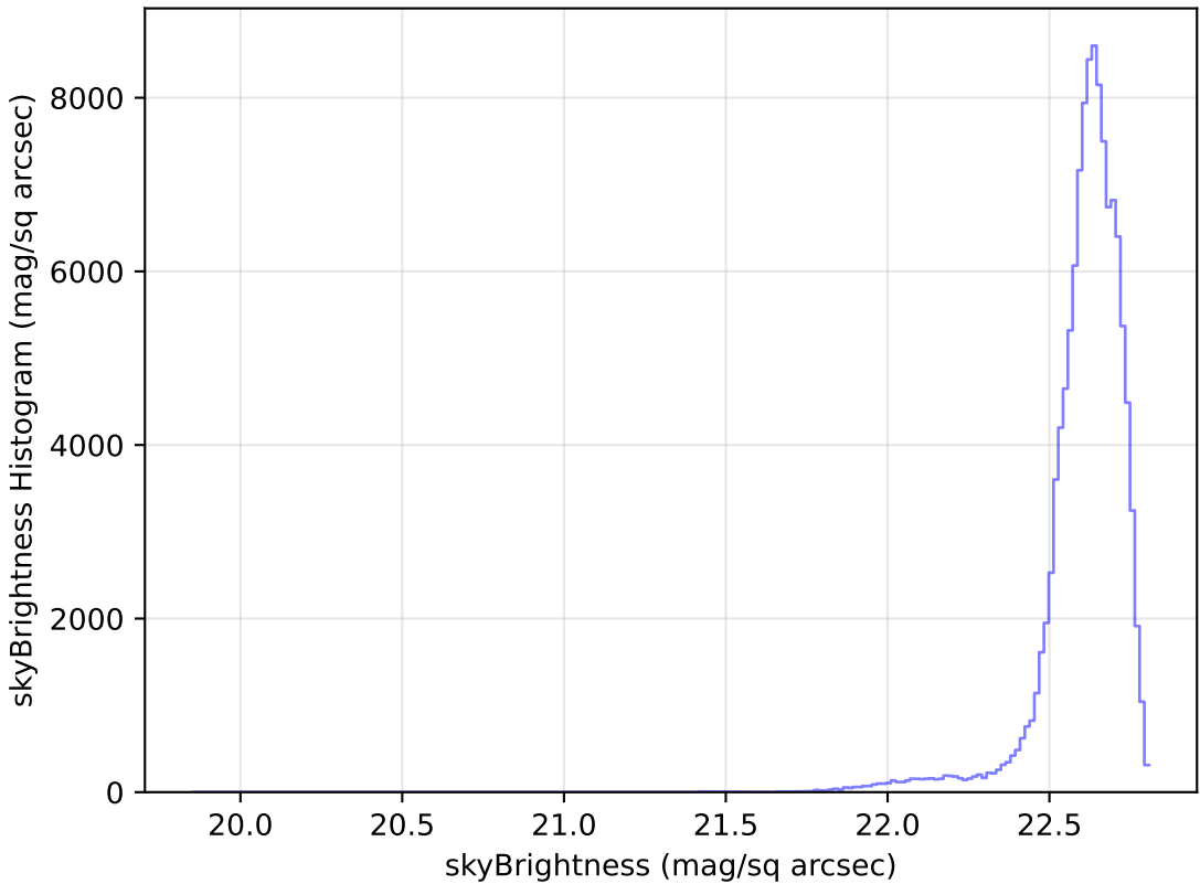
too_elab_r8_d3_ugrizy_v3.4_10yrs WFD u band: skyBrightness Histogram
