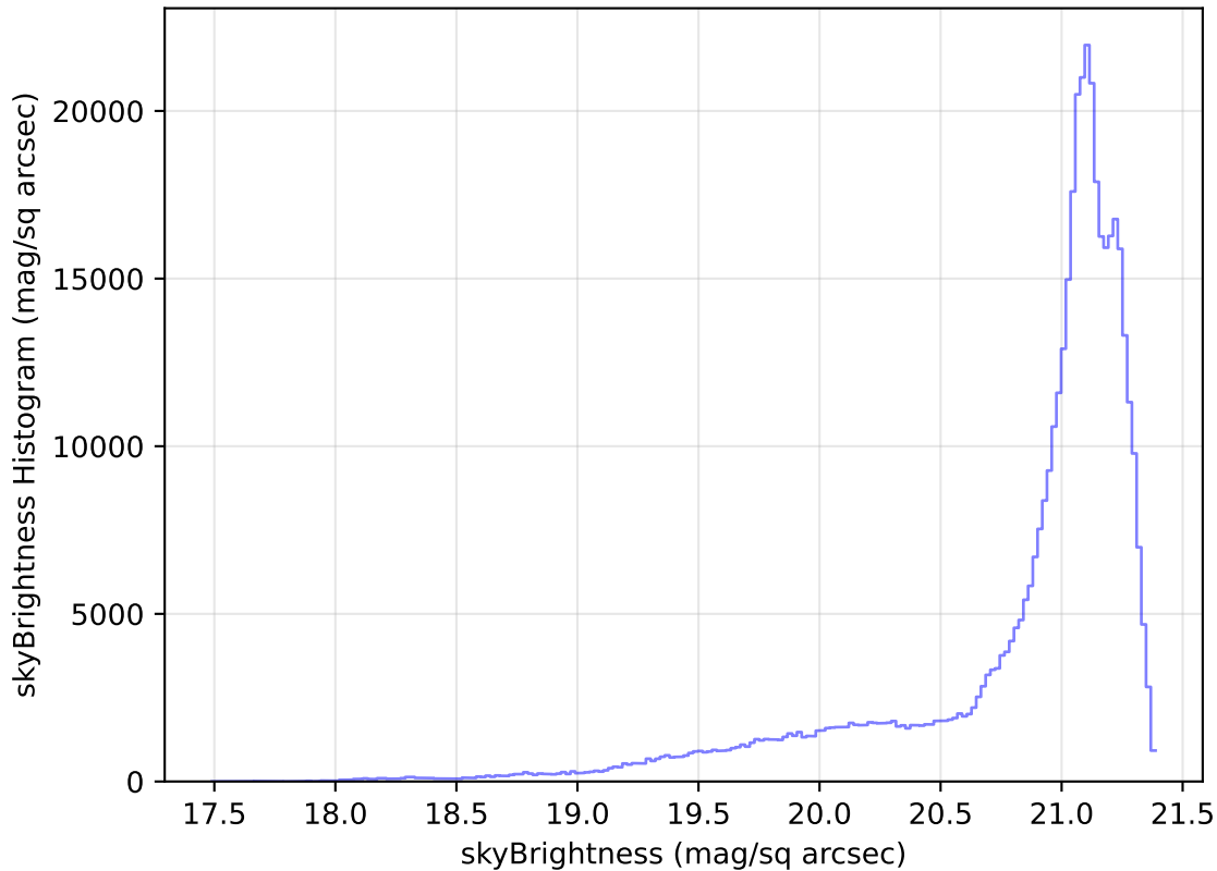
too_elab_r8_d3_ugrizy_v3.4_10yrs WFD r band: skyBrightness Histogram
