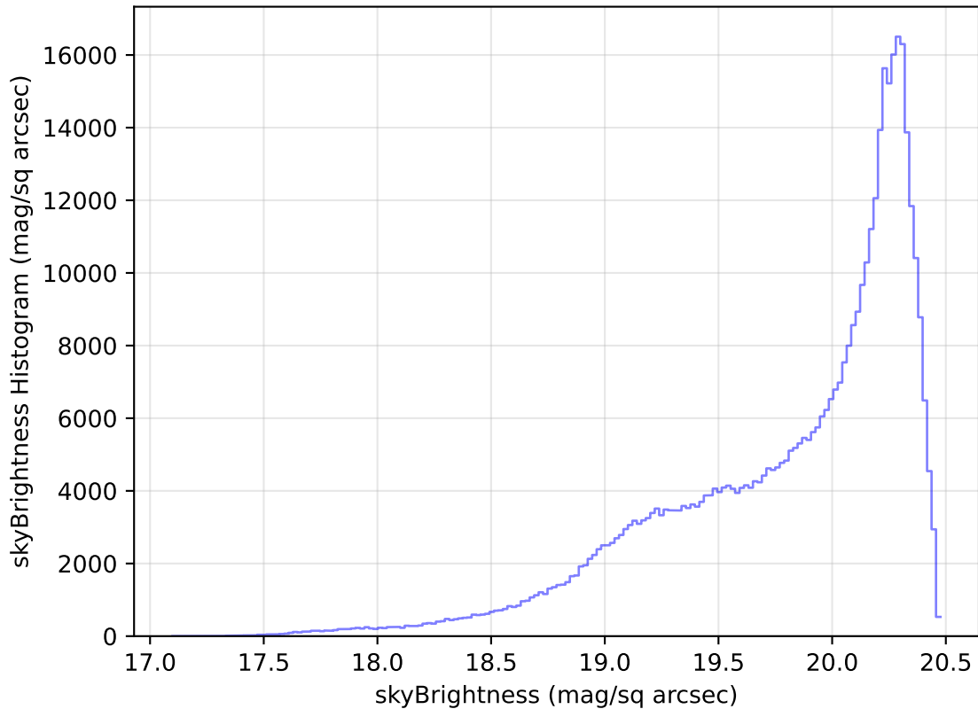
too_elab_r8_d3_ugrizy_v3.4_10yrs WFD i band: skyBrightness Histogram
