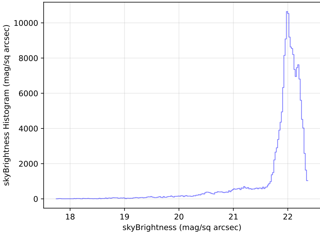
too_elab_r8_d3_ugrizy_v3.4_10yrs WFD g band: skyBrightness Histogram
