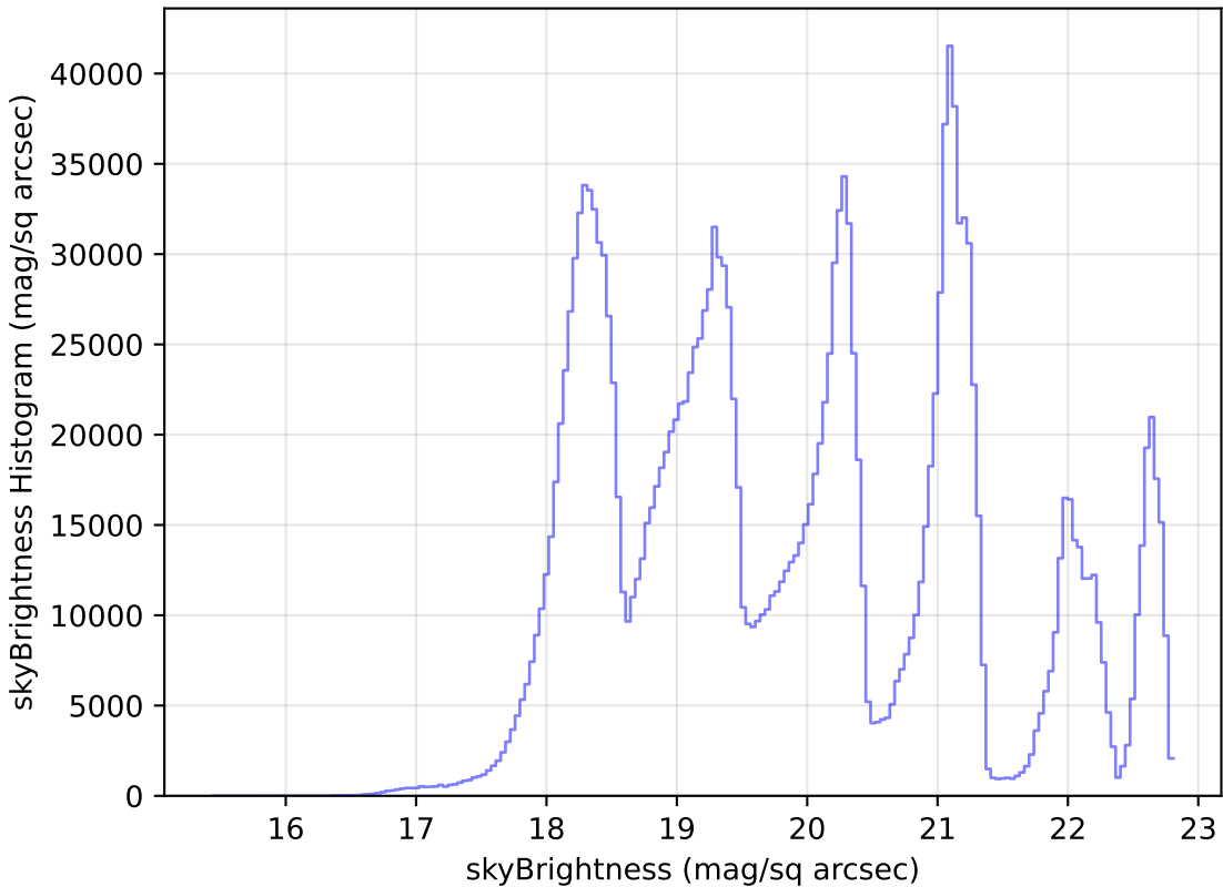
too_elab_r8_d3_ugrizy_v3.4_10yrs WFD all bands: skyBrightness Histogram
