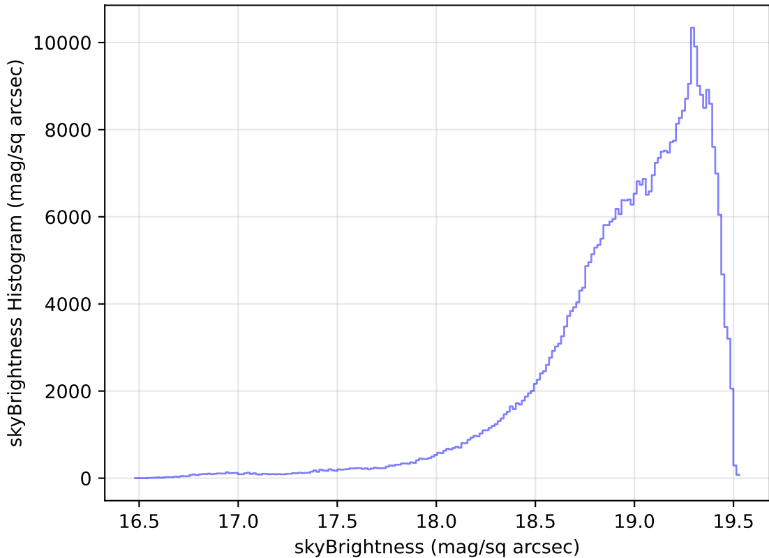
too_elab_r8_d3_ugrizy_v3.4_10yrs All sky z band: skyBrightness Histogram
