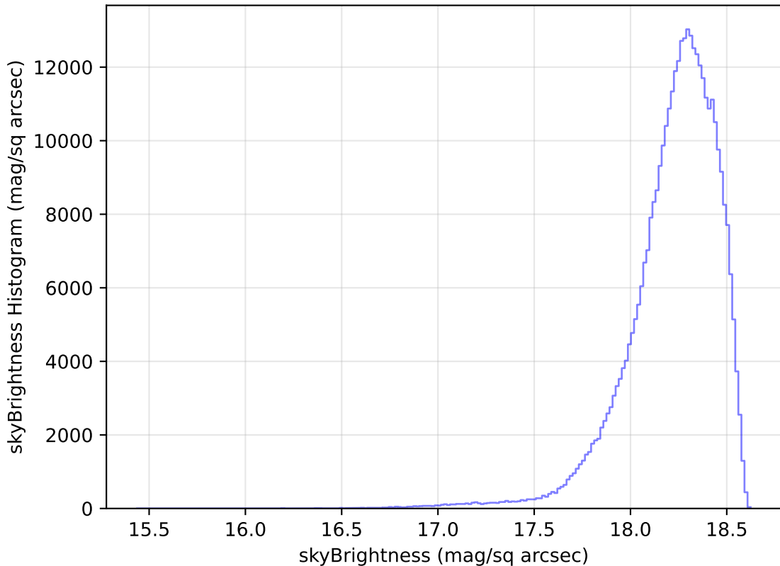
too_elab_r8_d3_ugrizy_v3.4_10yrs All sky y band: skyBrightness Histogram
