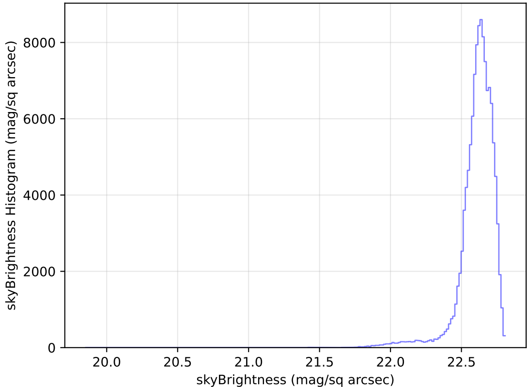
too_elab_r8_d3_ugrizy_v3.4_10yrs All sky u band: skyBrightness Histogram
