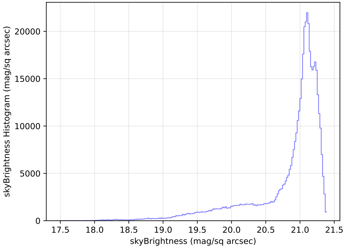
too_elab_r8_d3_ugrizy_v3.4_10yrs All sky r band: skyBrightness Histogram
