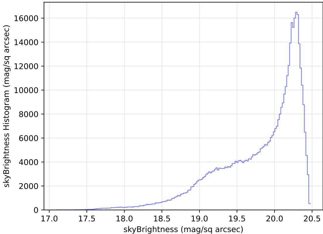
too_elab_r8_d3_ugrizy_v3.4_10yrs All sky i band: skyBrightness Histogram
