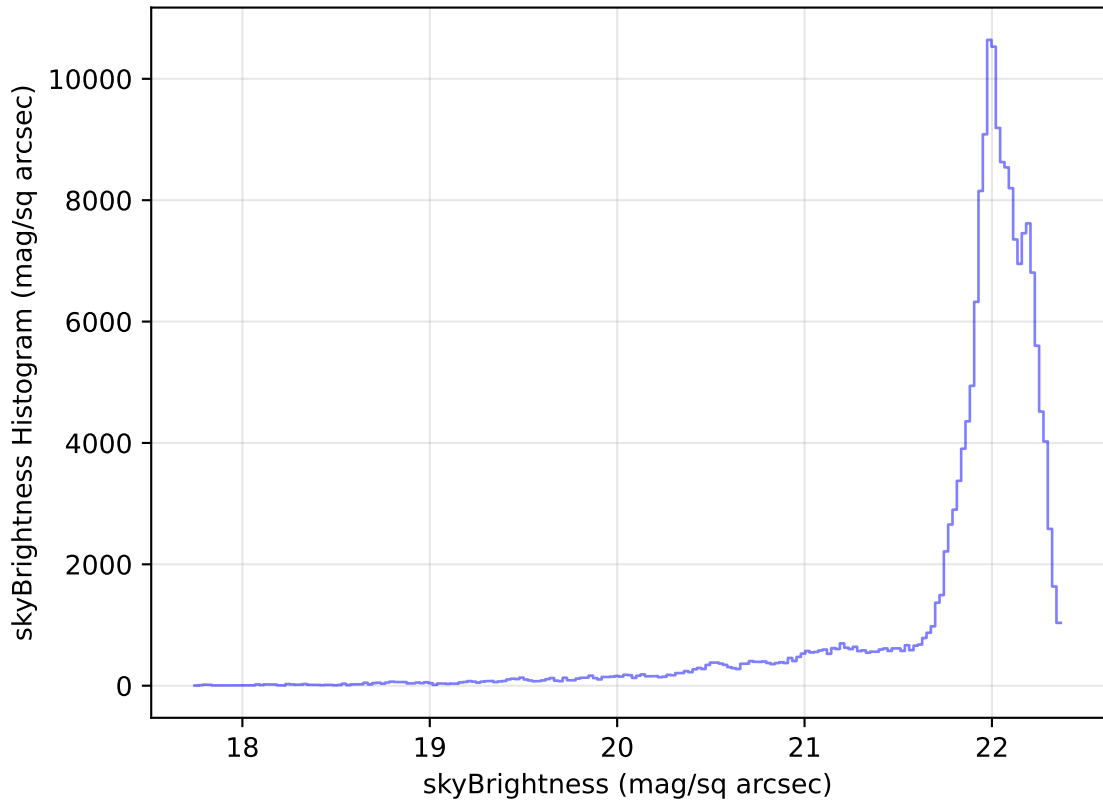
too_elab_r8_d3_ugrizy_v3.4_10yrs All sky g band: skyBrightness Histogram
