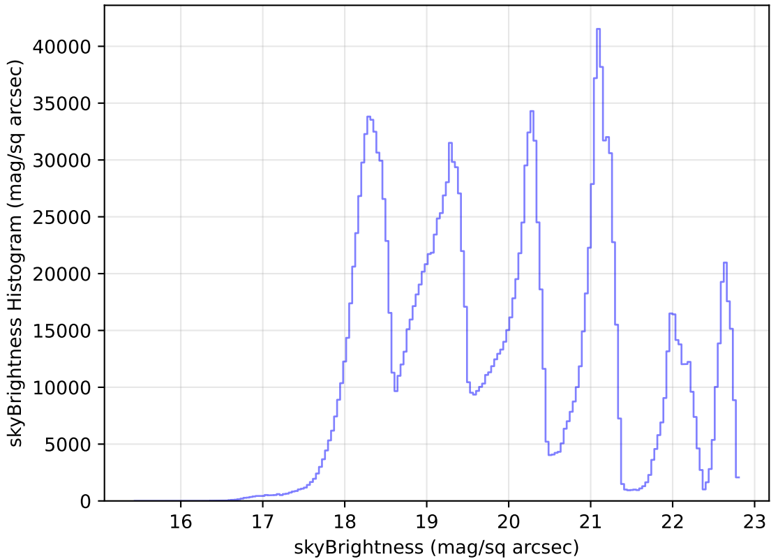
too_elab_r8_d3_ugrizy_v3.4_10yrs All sky all bands: skyBrightness Histogram
