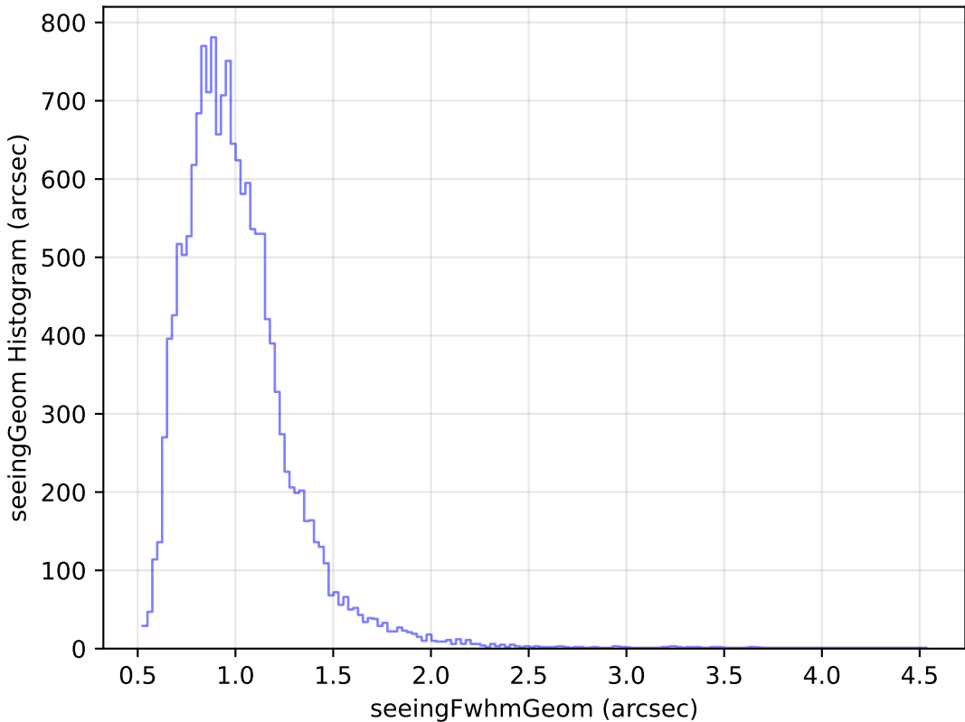
too_elab_r8_d3_ugrizy_v3.4_10yrs Yr 1 u band: seeingGeom Histogram
