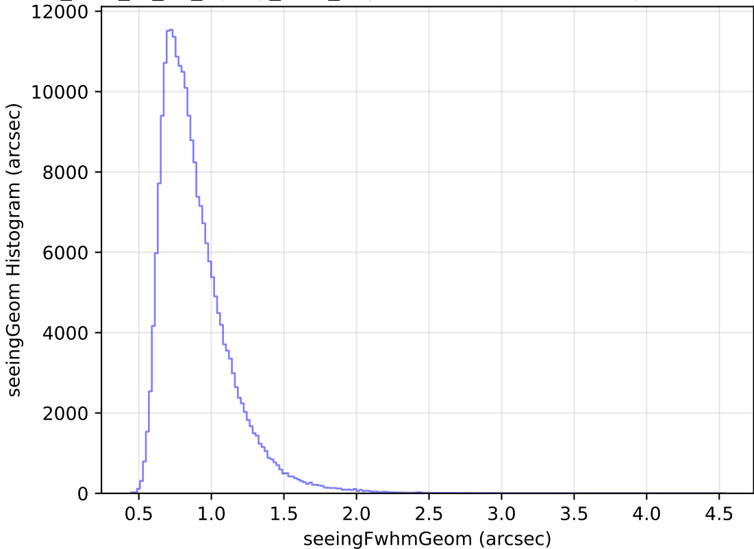
too_elab_r8_d3_ugrizy_v3.4_10yrs Yr 1 all bands: seeingGeom Histogram
