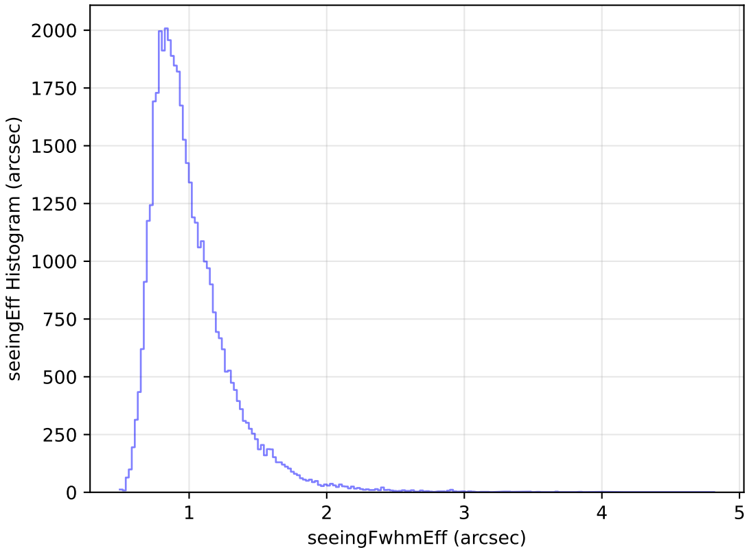
too_elab_r8_d3_ugrizy_v3.4_10yrs Yr 1 z band: seeingEff Histogram
