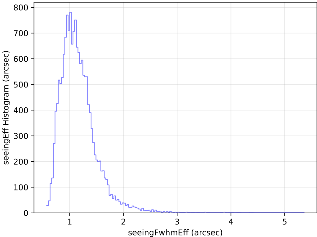
too_elab_r8_d3_ugrizy_v3.4_10yrs Yr 1 u band: seeingEff Histogram
