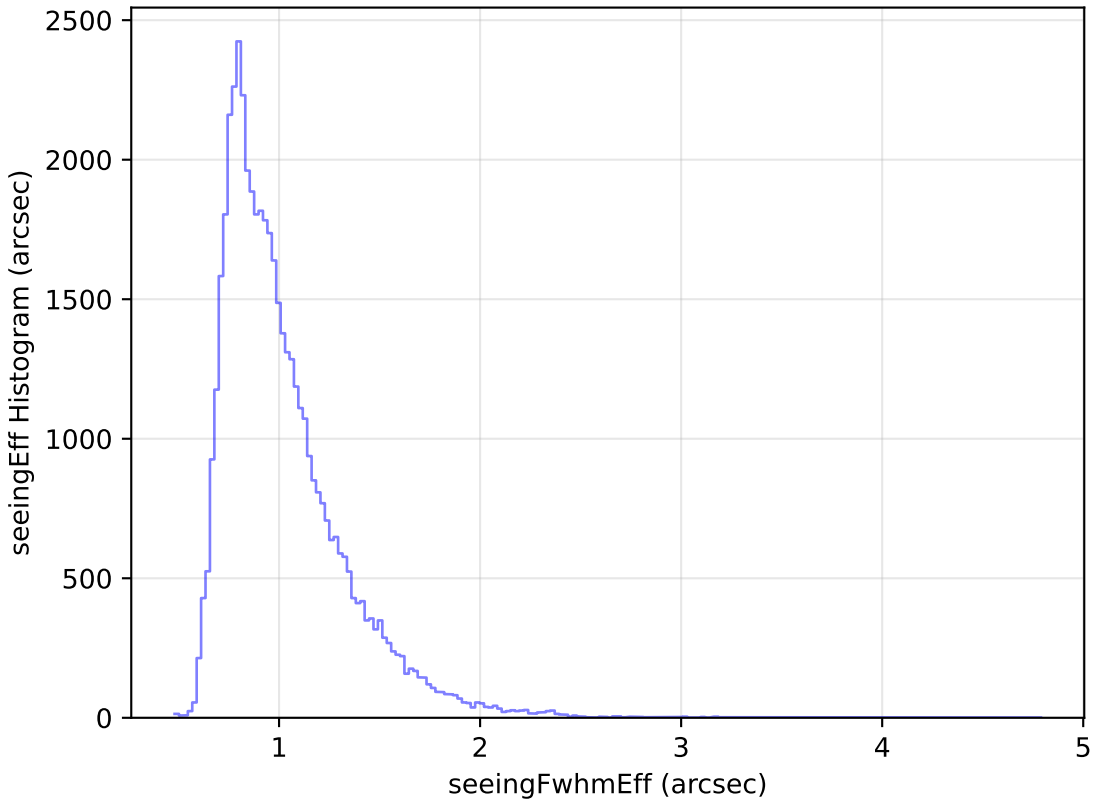
too_elab_r8_d3_ugrizy_v3.4_10yrs Yr 1 r band: seeingEff Histogram
