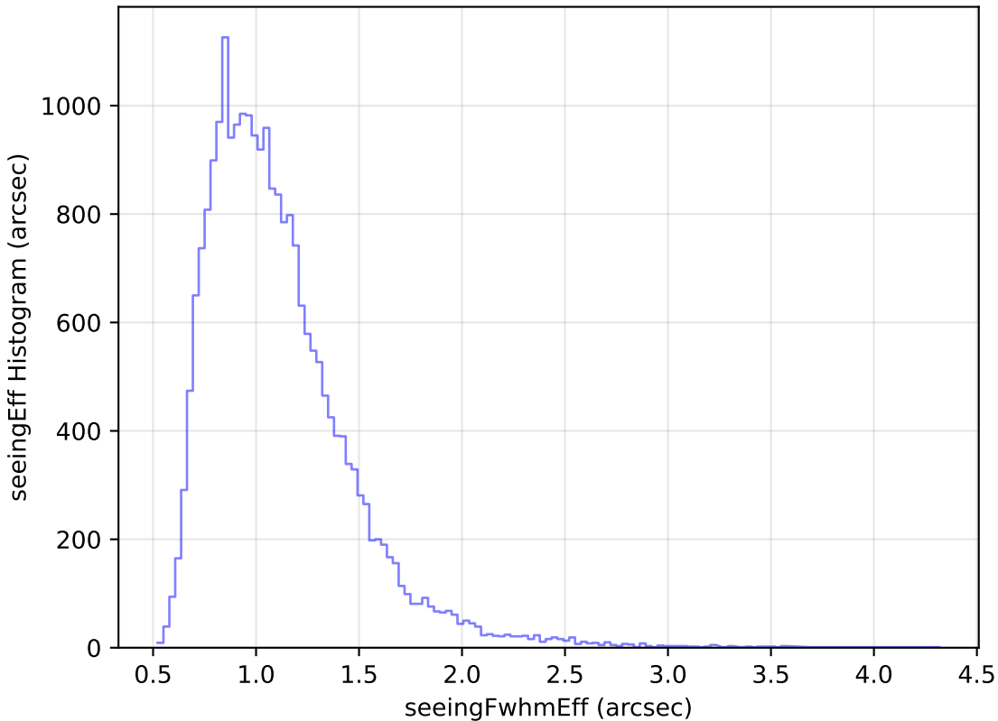
too_elab_r8_d3_ugrizy_v3.4_10yrs Yr 1 g band: seeingEff Histogram
