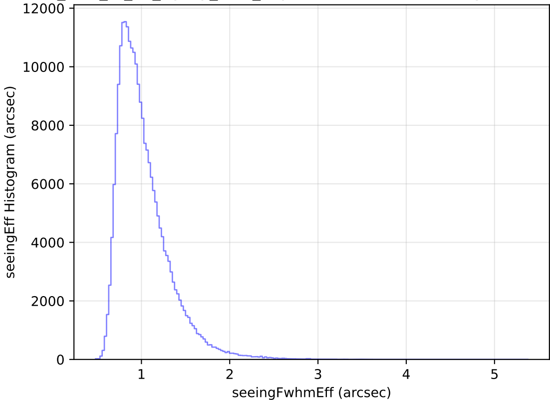
too_elab_r8_d3_ugrizy_v3.4_10yrs Yr 1 all bands: seeingEff Histogram
