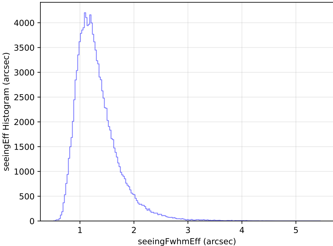
too_elab_r8_d3_ugrizy_v3.4_10yrs WFD u band: seeingEff Histogram
