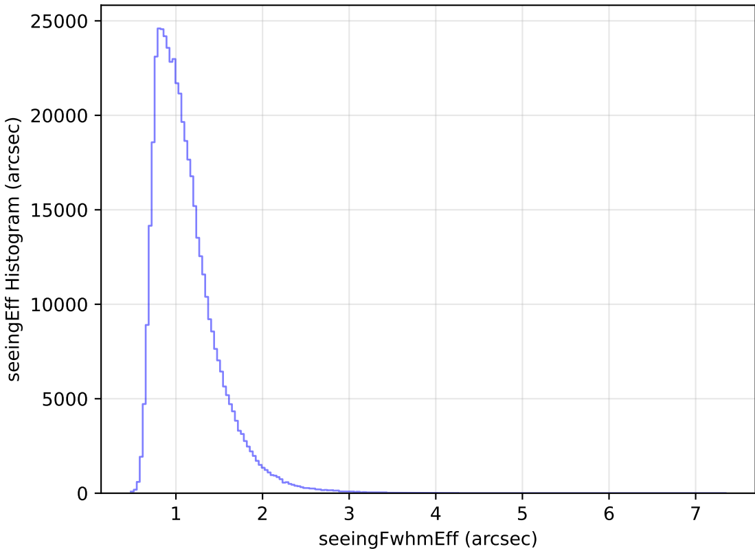
too_elab_r8_d3_ugrizy_v3.4_10yrs WFD r band: seeingEff Histogram
