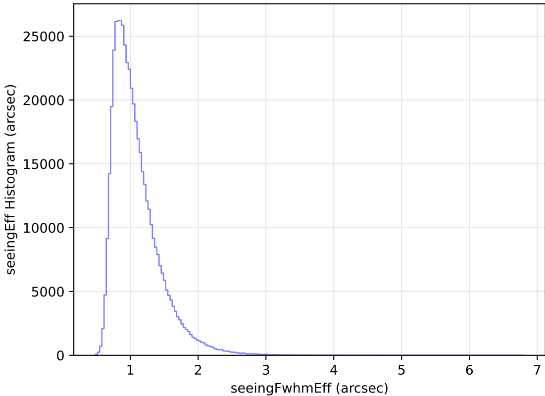
too_elab_r8_d3_ugrizy_v3.4_10yrs WFD i band: seeingEff Histogram
