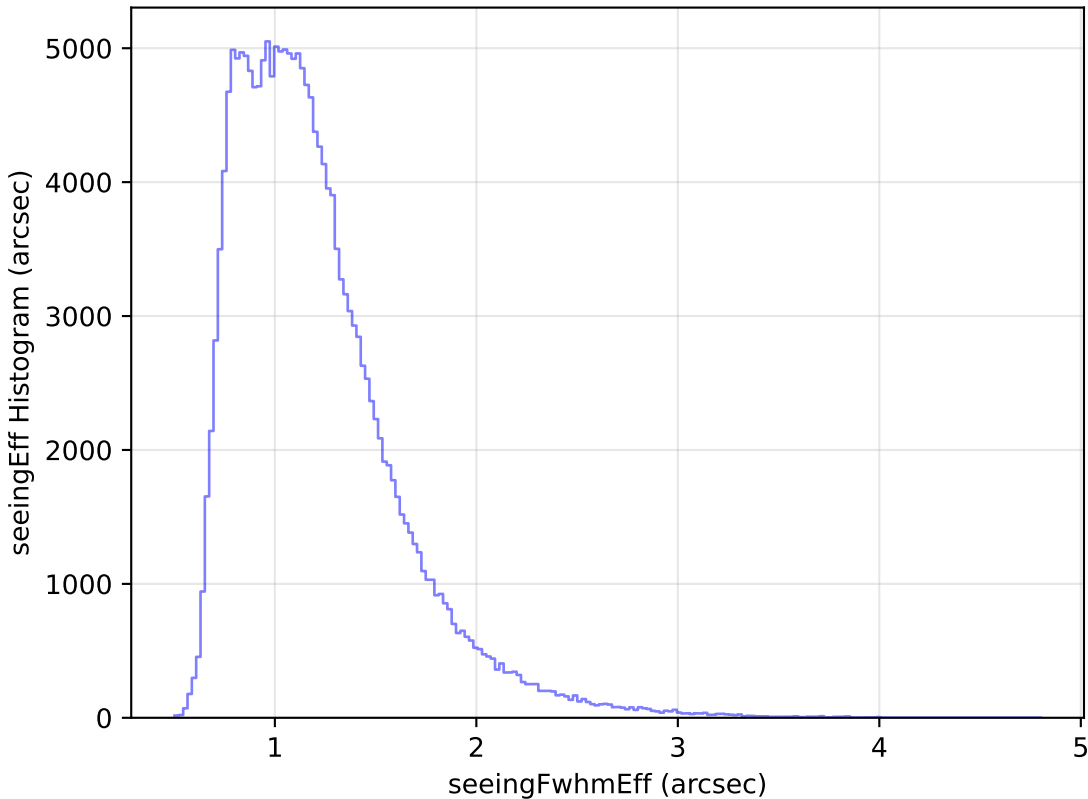
too_elab_r8_d3_ugrizy_v3.4_10yrs WFD g band: seeingEff Histogram
