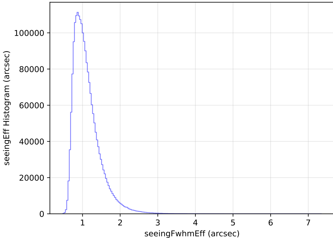
too_elab_r8_d3_ugrizy_v3.4_10yrs WFD all bands: seeingEff Histogram
