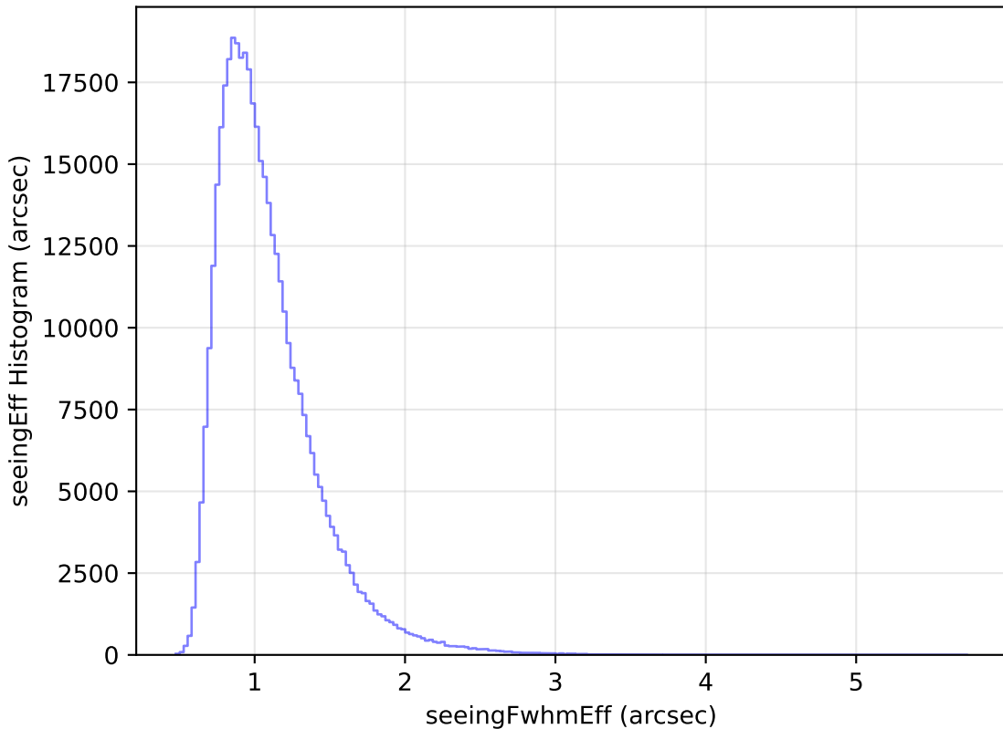
too_elab_r8_d3_ugrizy_v3.4_10yrs All sky z band: seeingEff Histogram
