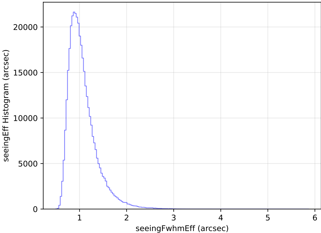
too_elab_r8_d3_ugrizy_v3.4_10yrs All sky y band: seeingEff Histogram
