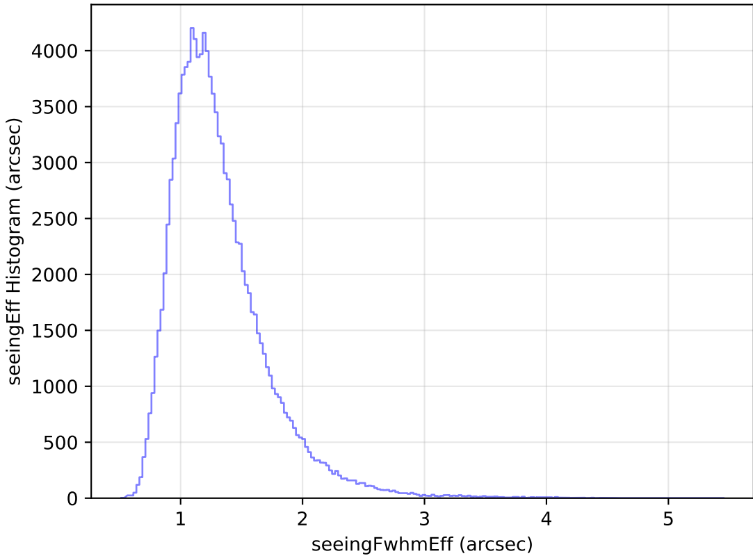
too_elab_r8_d3_ugrizy_v3.4_10yrs All sky u band: seeingEff Histogram
