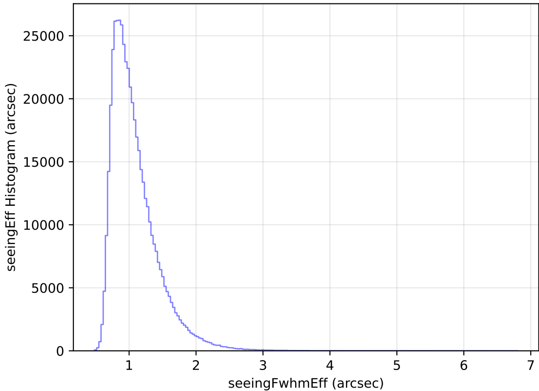
too_elab_r8_d3_ugrizy_v3.4_10yrs All sky i band: seeingEff Histogram
