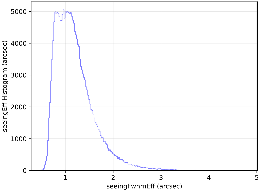
too_elab_r8_d3_ugrizy_v3.4_10yrs All sky g band: seeingEff Histogram
