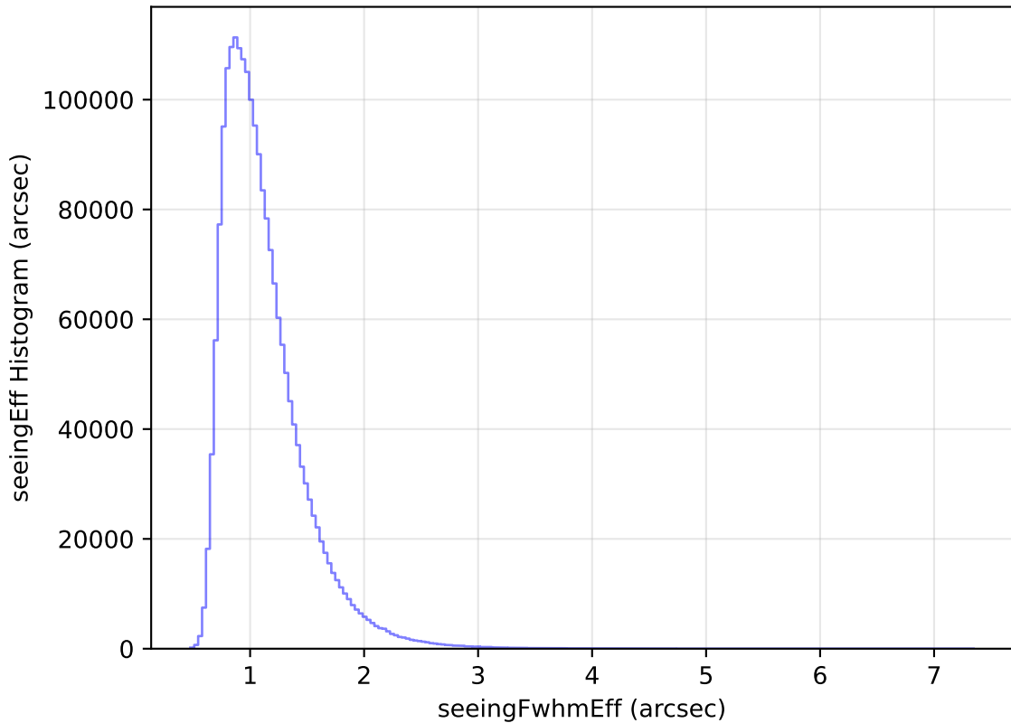
too_elab_r8_d3_ugrizy_v3.4_10yrs All sky all bands: seeingEff Histogram
