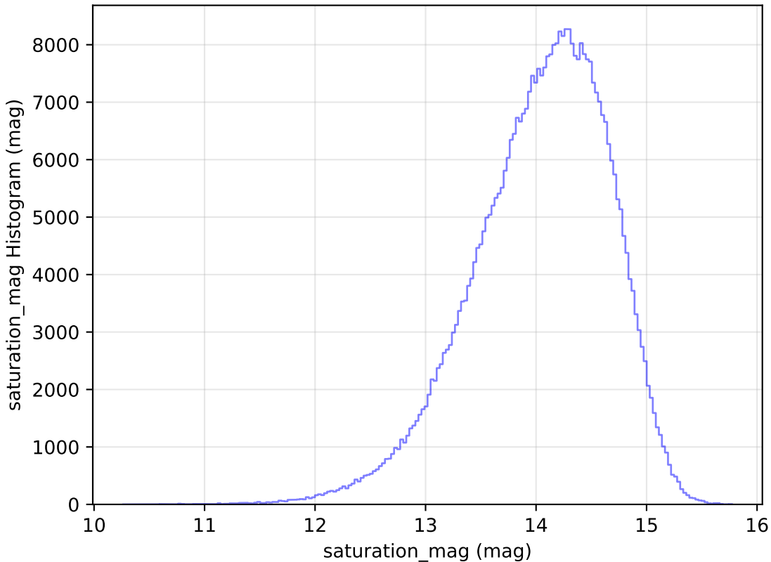
too_elab_r8_d3_ugrizy_v3.4_10yrs WFD z band: saturation_mag Histogram
