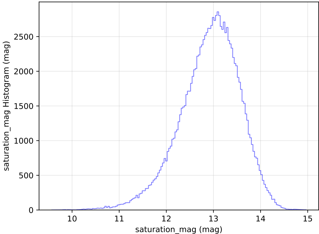
too_elab_r8_d3_ugrizy_v3.4_10yrs WFD u band: saturation_mag Histogram
