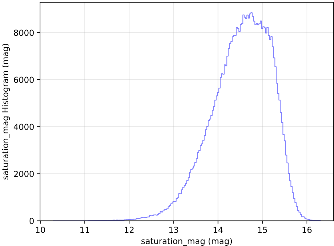
too_elab_r8_d3_ugrizy_v3.4_10yrs WFD r band: saturation_mag Histogram
