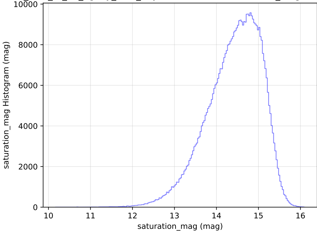
too_elab_r8_d3_ugrizy_v3.4_10yrs WFD i band: saturation_mag Histogram
