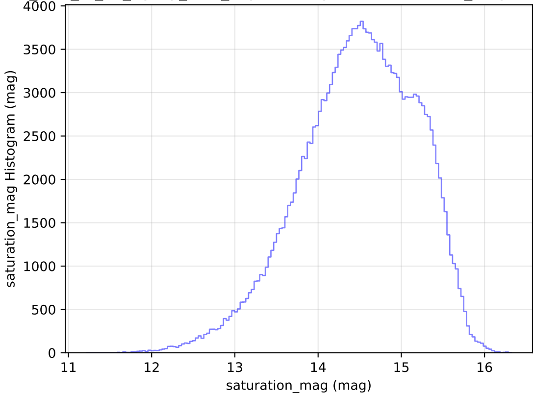
too_elab_r8_d3_ugrizy_v3.4_10yrs WFD g band: saturation_mag Histogram
