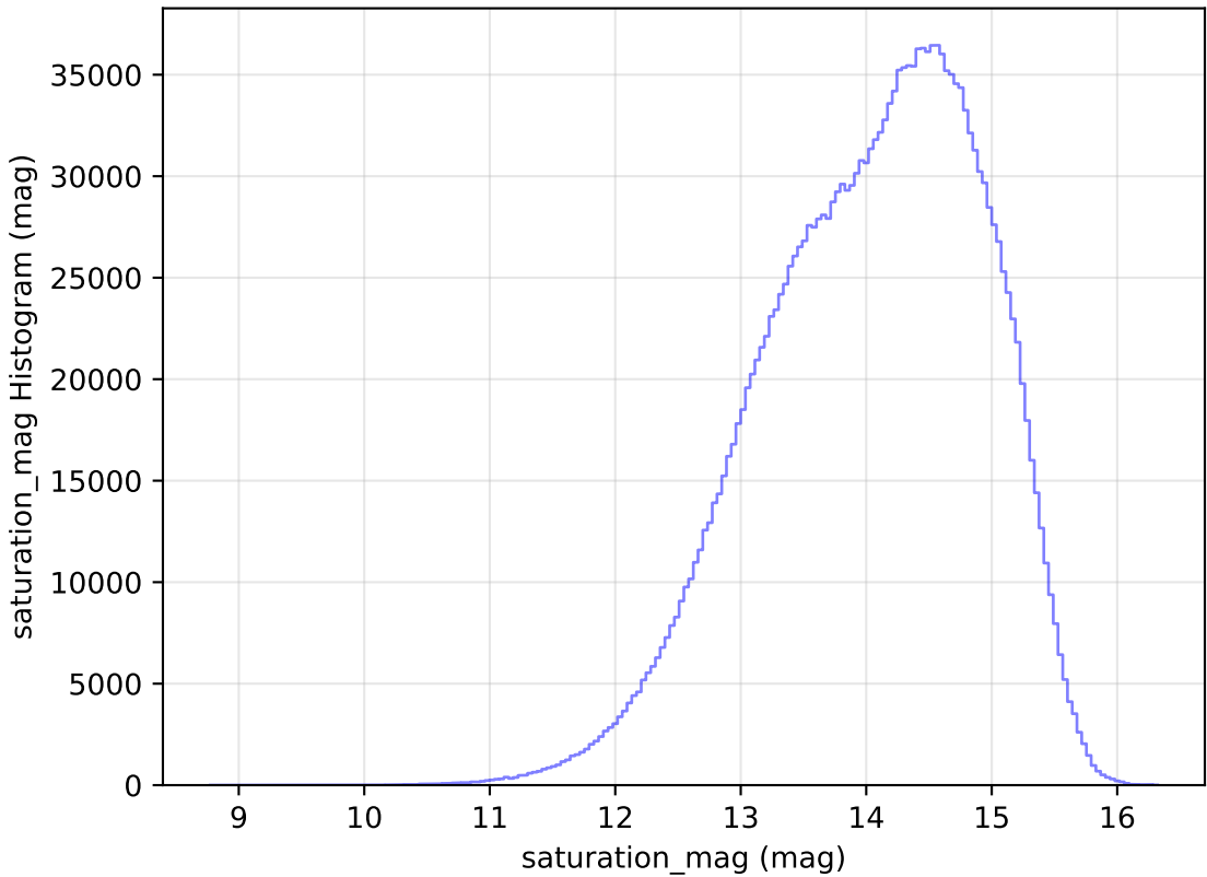
too_elab_r8_d3_ugrizy_v3.4_10yrs WFD all bands: saturation_mag Histogram
