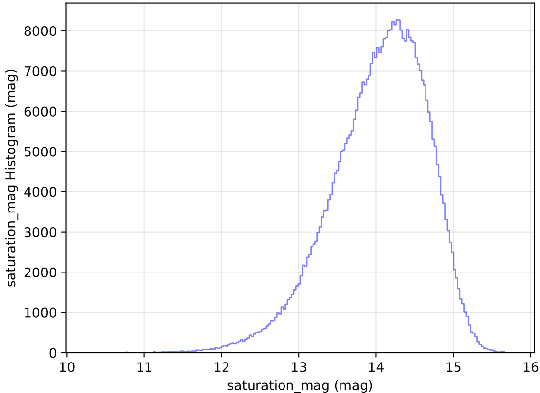
too_elab_r8_d3_ugrizy_v3.4_10yrs All sky z band: saturation_mag Histogram
