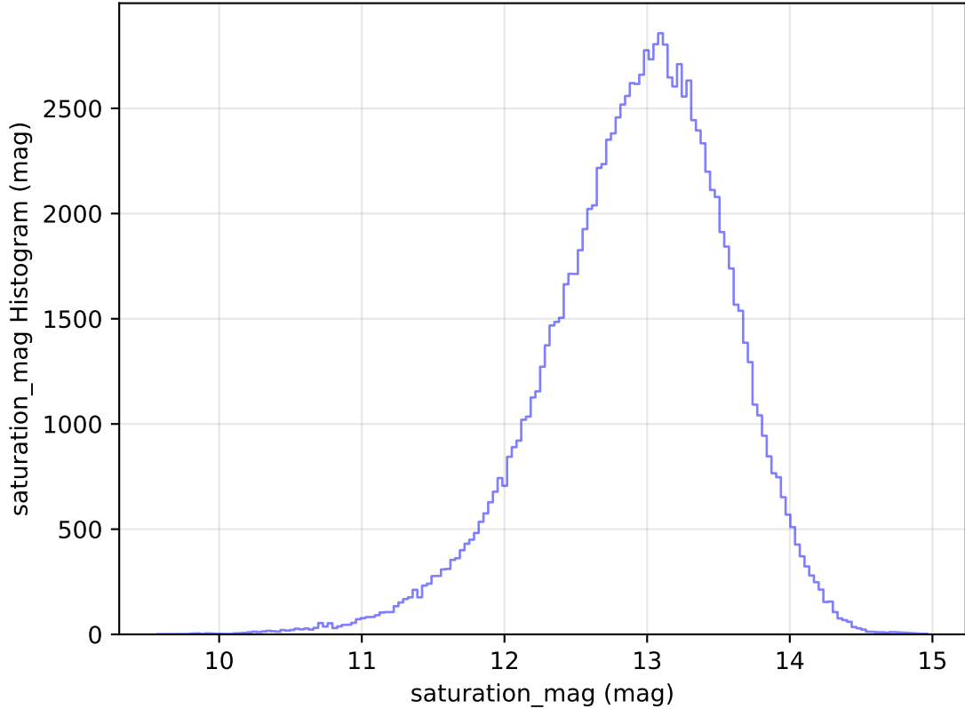
too_elab_r8_d3_ugrizy_v3.4_10yrs All sky u band: saturation_mag Histogram
