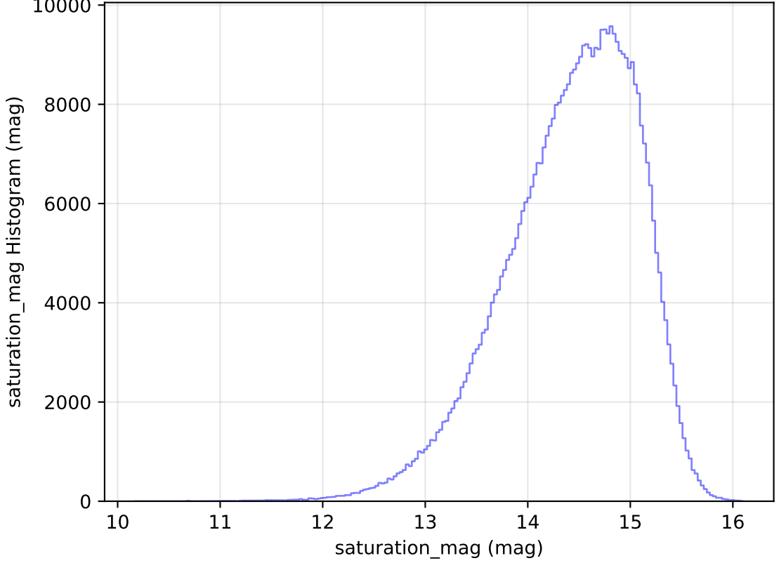
too_elab_r8_d3_ugrizy_v3.4_10yrs All sky i band: saturation_mag Histogram
