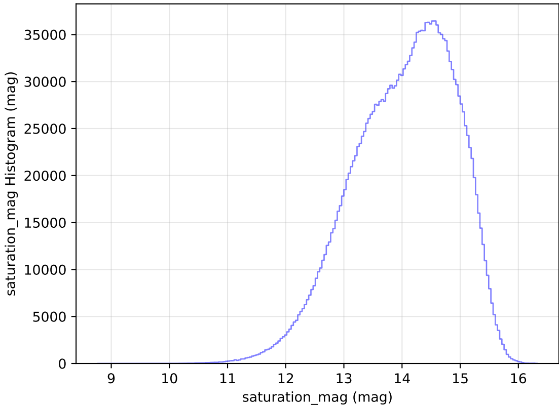
too_elab_r8_d3_ugrizy_v3.4_10yrs All sky all bands: saturation_mag Histogram
