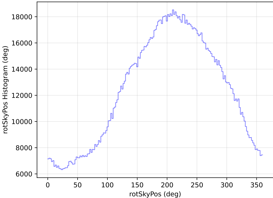
too_elab_r8_d3_ugrizy_v3.4_10yrs WFD all bands: rotSkyPos Histogram
