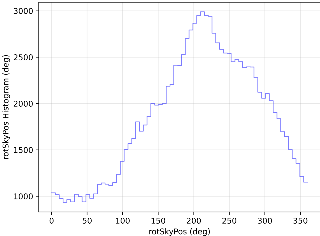
too_elab_r8_d3_ugrizy_v3.4_10yrs All sky u band: rotSkyPos Histogram
